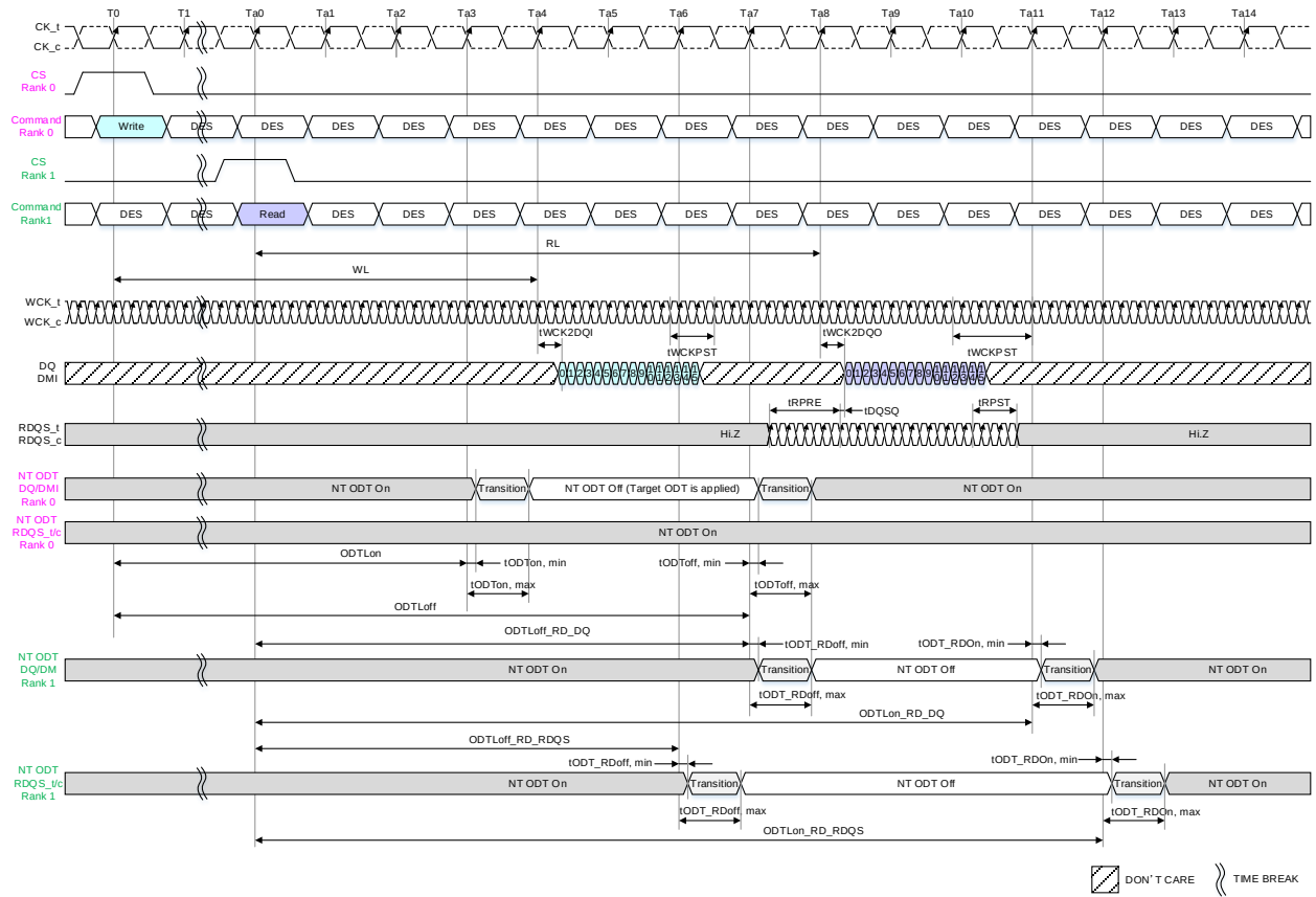
Figure 209 — Write to Read Rank2Rank Operation (MR0 OP[0]=1B)
