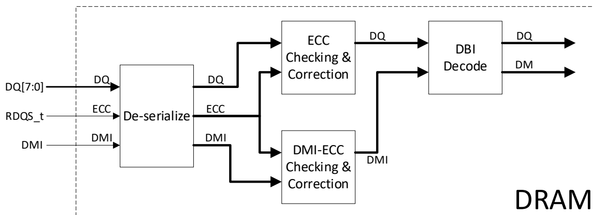
Figure 266 — Data flow on a memory Write operation
